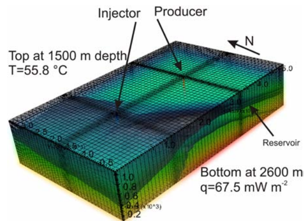
Figure 10: Sketch of the reservoir model, showing the grid and the layers, as well as the position of the producer and injector. The grid is refined at these locations. The y-axis is rotated by 8 degrees from north counterclockwise.
